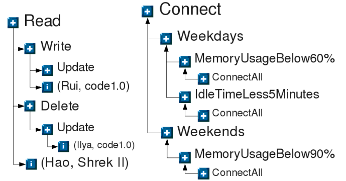
Fig. 3. Permission Hierarchies.
