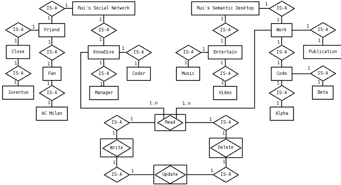
Fig. 4. A portion of the ER Diagram of Figures 2,3.
